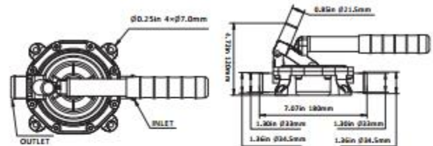
SFDHA-G720-01 Aluminium Handle
